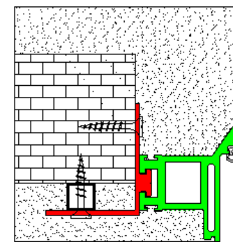
Brick wall
