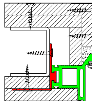
Plasterboard wall
